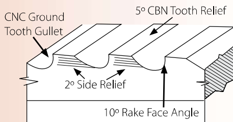
Davis Keyseat Puller Design
